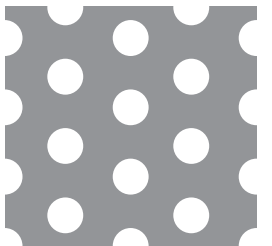
3/16" DIA 3/8" CTRS 23% OPEN AREA
