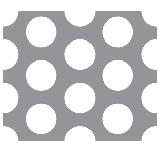
5/16" DIA 7/16" CTRS 46% OPEN AREA
