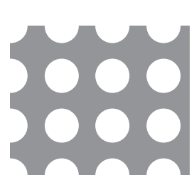
1/4" DIA 3/8" CTRS 35% OPEN AREA
