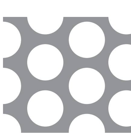
5/8" DIA 7/8" CTRS 46% OPEN AREA
