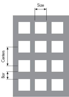
STRAIGHT LINE SQUARE PERFORATIONS
