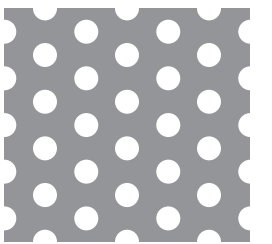
1/8" DIA 1/4" CTRS 23% OPEN AREA
