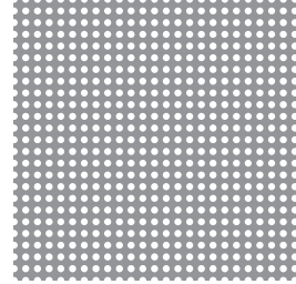
.033" DIA .055" CTRS 33% OPEN AREA
