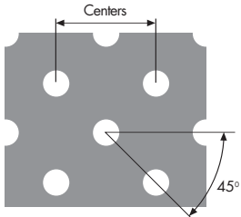
OPTIONAL ROUND PERFORATIONS 45° STAGGERED
